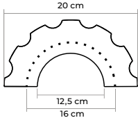
C3002H H: 239,5 cm ProFoam®
